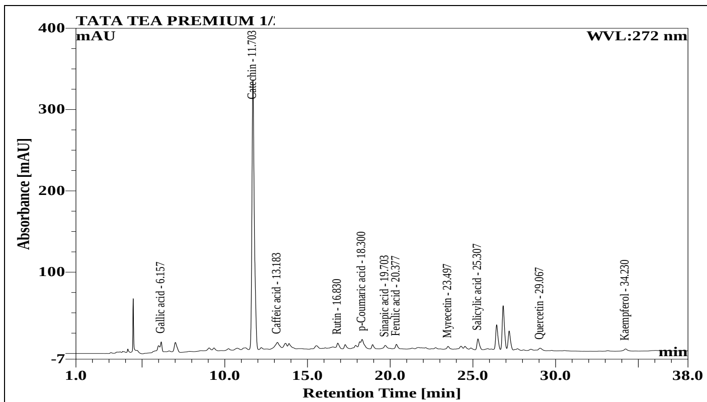
Fig. 2: HPLC chromatogram of black tea
