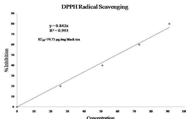
Fig. 1: DPPH radical scavenging activity of black tea
