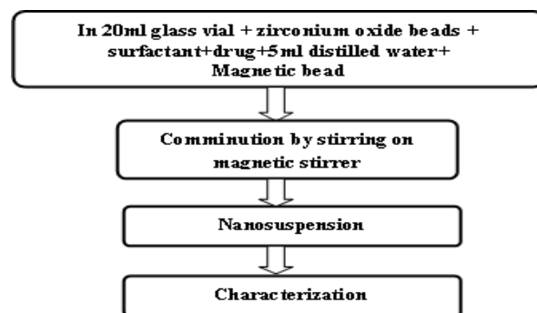
Fig. 1: Flow chart for preparation of metaxalone nanosuspension
