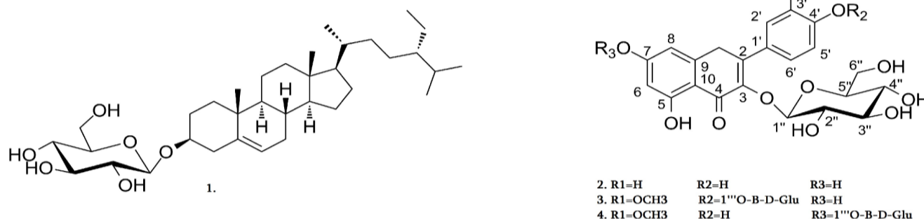
Fig. 1: Chemical structures of compound 1, 2, 3, 4.
