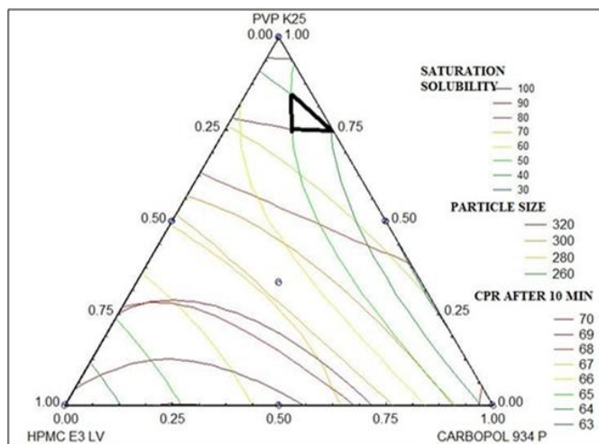
Fig. 6: Overlay counter plot for all dependent variables.
