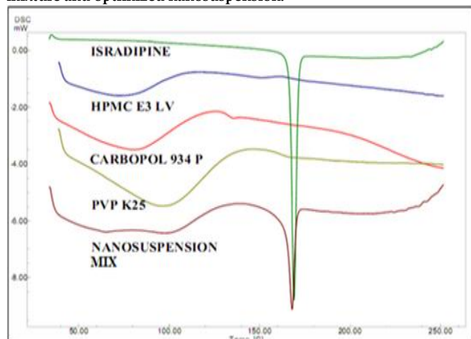
Fig. 11: Overlay of DSC thermograms of Isradipine, HPMC E3 LV, Carbopol 934P, PVP K25 and physical mixture of nanosuspension.
