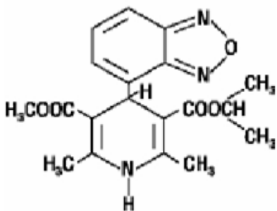
Fig. 1: Structure of Isradipine
