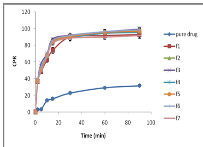
Fig. 9: Comparison of dissolution profile of all batches of simplex lattice design with pure drug.
