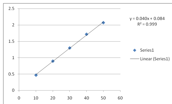
Fig. 1: Calibration curve of Ondansetron hydrochloride
