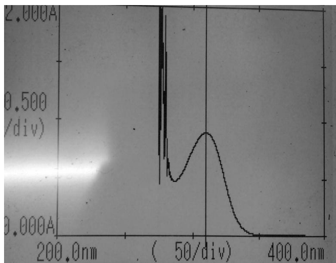
Fig. 2: UV-Spectrum of Ondansetron hydrochloride
