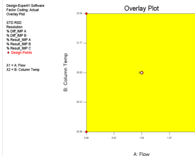
Fig. 4: Design space overlay plot
