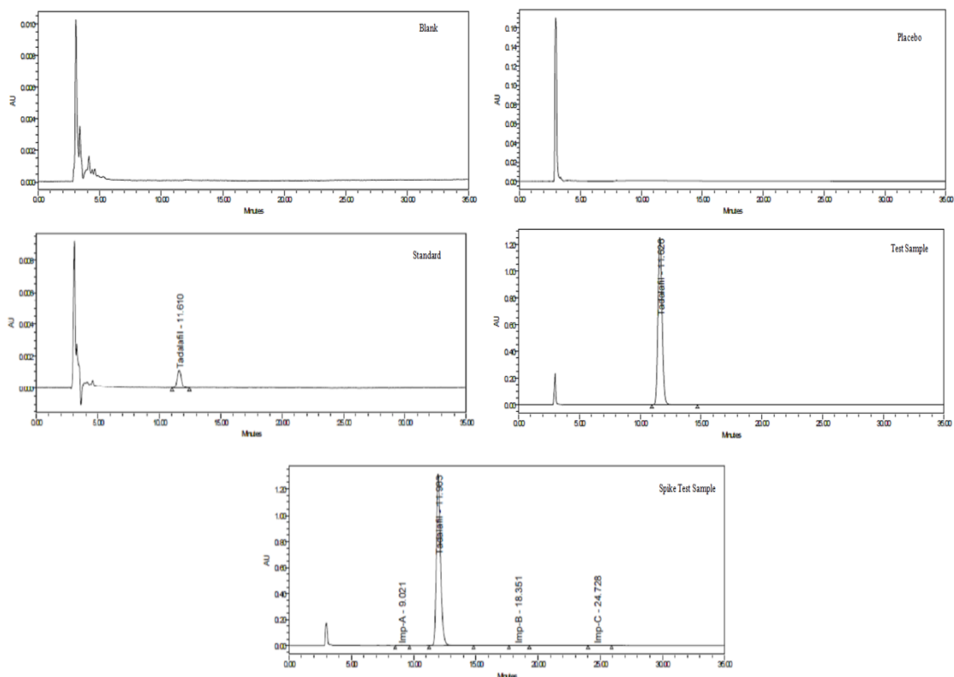
Fig. 3: Chromatograms of tadalafil and its impurities.
