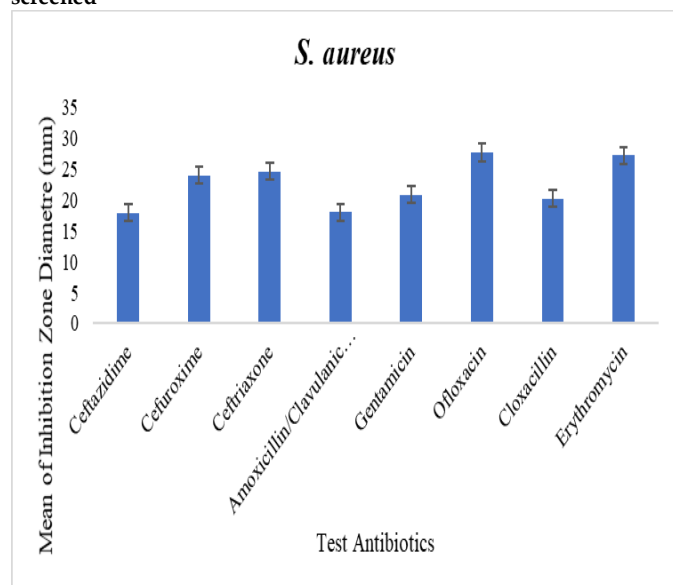
Fig. 4: Antibiogram summary for Staphylococcus aureus .
