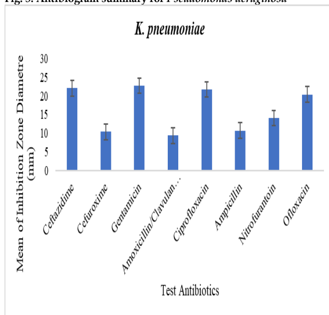
Fig. 6: Antibiogram summary for Klebsiella pneumoniae .
