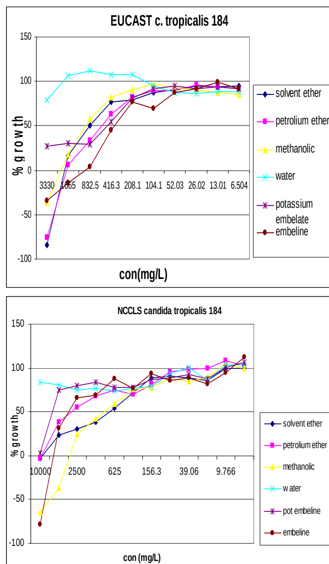
Fig. 1: Extract concentration against percentage growth of C. tropicalis for EUCAST and NCCLS method.
