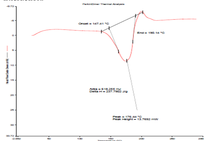
Fig. 5: DSC thermogram of Ciprofloxacin HCl
