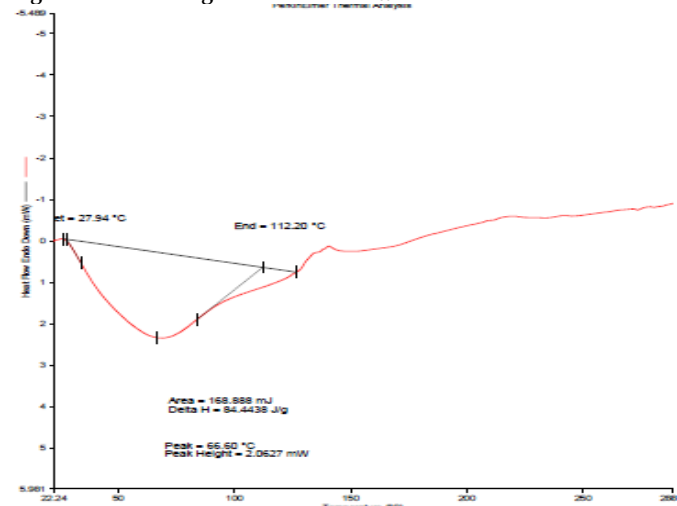
Fig. 7: DSC thermogram of Ethyl Cellulose
