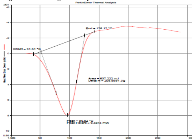
Fig. 6: DSC thermogram of HPMC K 100 M
