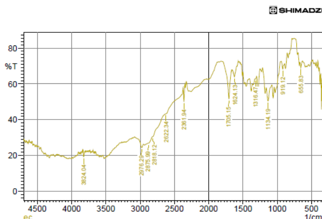
Fig. 3: FTIR Spectra of Ethyl Cellulose
