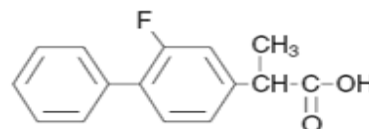
Fig. 1: Structure of Flurbiprofen
