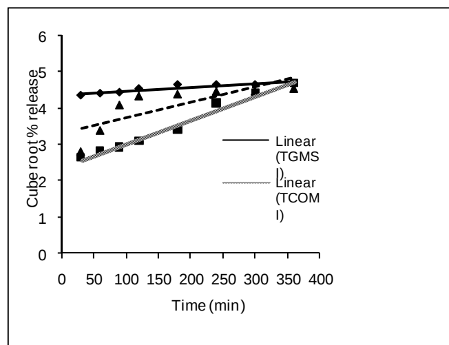
Fig. 4: Hixson-Crowell cube root plots of etoricoxib from the formulated tablets
