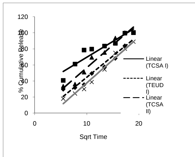
Fig. 3: Higuchi release model of etoricoxib hydrophobic matrix tablet formulations
