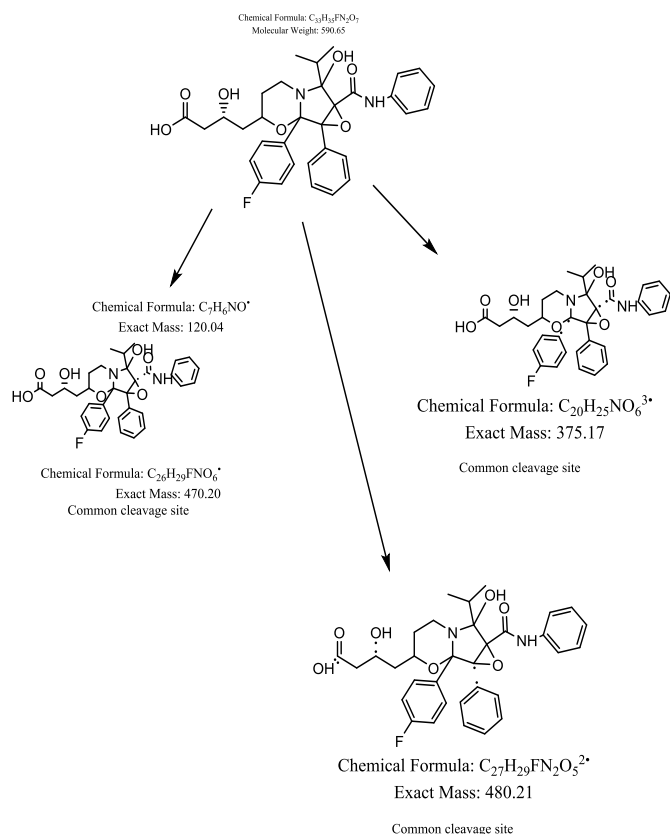
Fig. 5: MSMS fragmentation of unknown impurity at RRT-1.29
