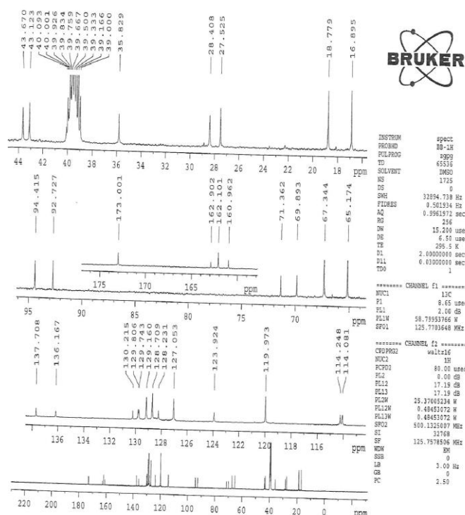
Fig. 10: 13 C NMR spectrum of unknown impurity
