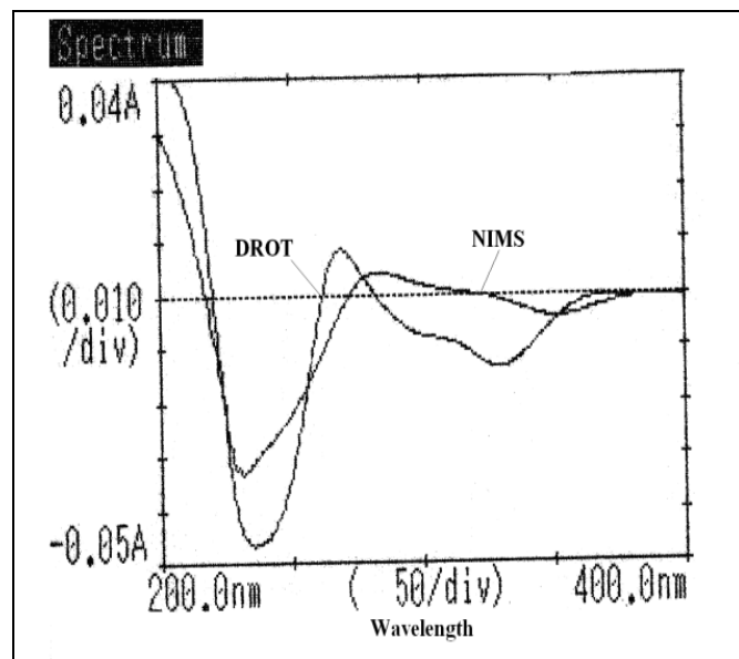
Fig. 1: First order derivative overlay spectra of NIMS and DROT
