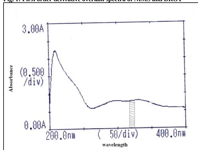
Fig. 1: First order derivative overlay spectra of NIMS and DROT
