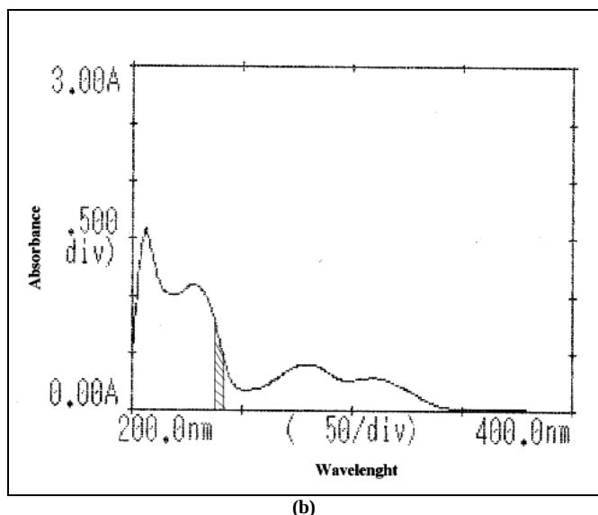
Fig. 2: UV spectra of (a) NIMS and (b) DROT along with AUC range
