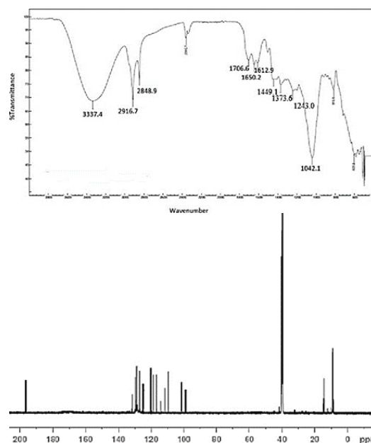
Fig. 8: IR and 13 C NMR graph of bonducellin
