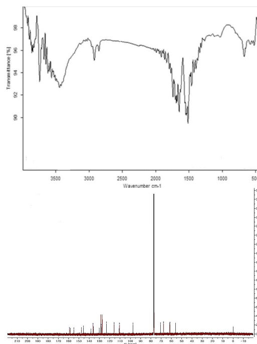
Fig. 7: IR and 13 C-NMR graph of caesalpinianone
