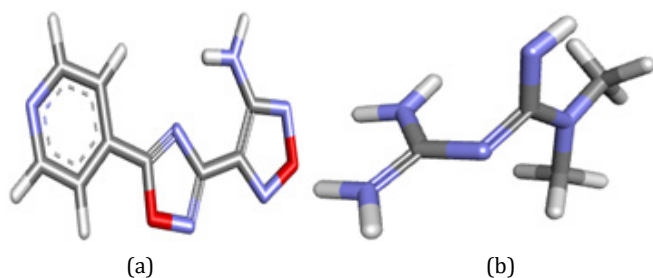
Fig. 1: a) Structure of ligand POA and b) Metformin (Drug molecule)
