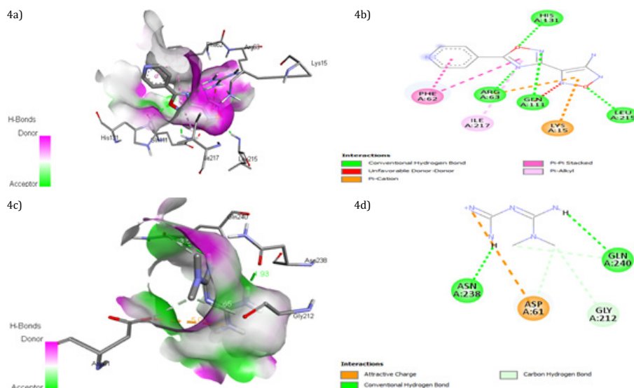
Fig. 4: Molecular binding of POA with human SIRT6 (PDB: 3K35). (4a) Interaction of POA with residues along with H-bonds donor and acceptor regions. (4b) 2D plot with POA (4c) Interaction of Metformin with residues along with H-bonds donor and acceptor regions. (4d) 2D plot with metformin
