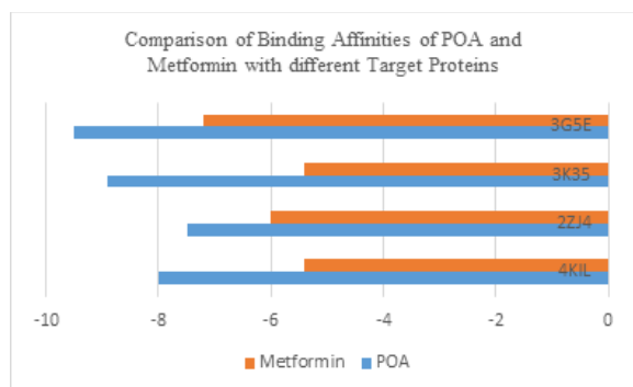
Fig. 7: Comparison of binding affinities of POA and metformin with different target proteins
