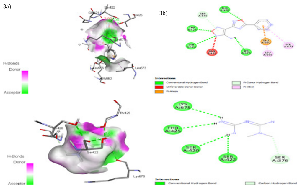
Fig. 3: Significant molecular bonding of POA and metformin with GFAT (PDB: 2ZJ4). (3a) Interaction of POA with residues along with H-bonds donor and acceptor regions. (3b) 2D plot POA (3c) Interaction of metformin with residues along with H-bonds donor and acceptor regions. (3d) 2D plot with metformin
