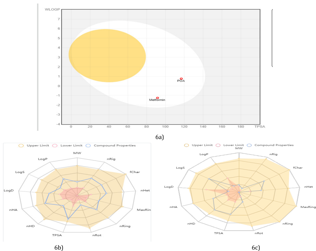
Fig. 6: (a) BOILED-Egg plot showing BBB penetration and HIA of POA and metformin molecules. (b) Radar graph* for POA (c) Radar graph* for metformin, *shows upper and lower range of various physicochemical and molecular properties with predicted values
