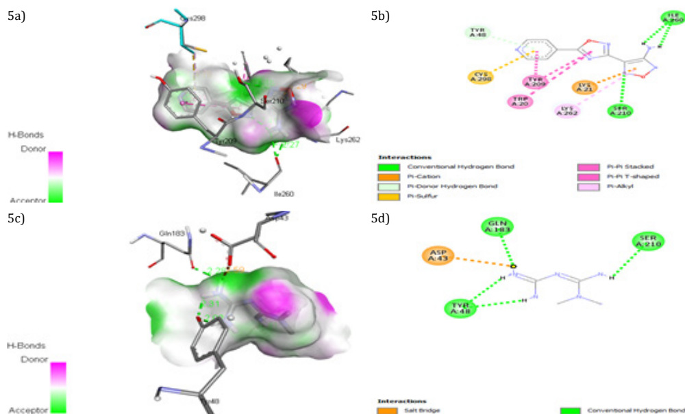
Fig. 5: Molecular binding of POA with 3G5E. (5a) POA interaction with residues, H-bonds donor, and acceptor regions. (5b) 2D plot with POA (5c) Interaction of Metformin with residues, H-bonds donor, and acceptor regions. (5d) 2D plot with metformin
