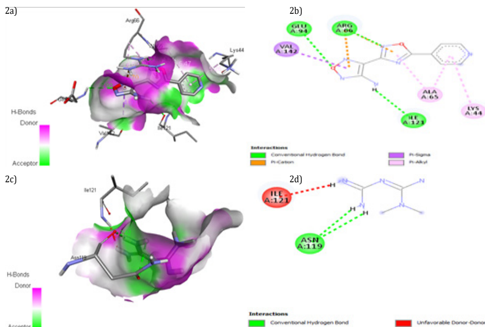
Fig 2: Molecular binding of POA and metformin with 11 β -HSD1 (PDB ID- 4K1L). (2a) Interaction of POA with residues along with H-bonds donor and acceptor regions. (2b) 2D plot with POA (2c) Interaction of metformin with residues along with H-bonds donor and acceptor regions. (2d) 2D plot with metformin
