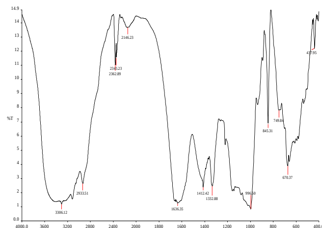
Fig. 6: FTIR spectrum of physical mixture of Isoniazid and sodium alginate
