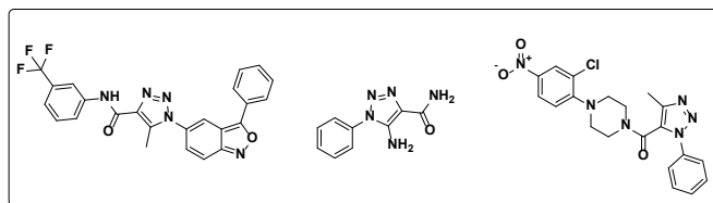
Fig. 1: Structures of some 1H-1,2,3-triazole-4-carboxamide derivatives with anticancer activity
