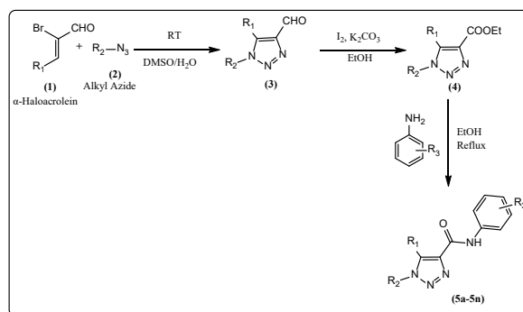
Fig. 2: Scheme of synthesis for 1,2,3-triazole carboxamide derivatives
