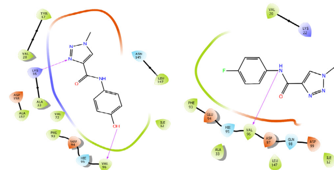
Fig. 4: Molecular interactions of compound 5f and 5g with the CDK4-Cyclin D3 (7SJ3) active site
