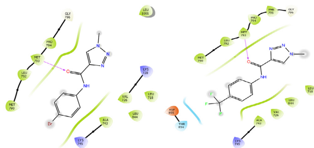
Fig. 3: Molecular interactions of compound 5i and 5j with the EGFR (6LUD) active site
