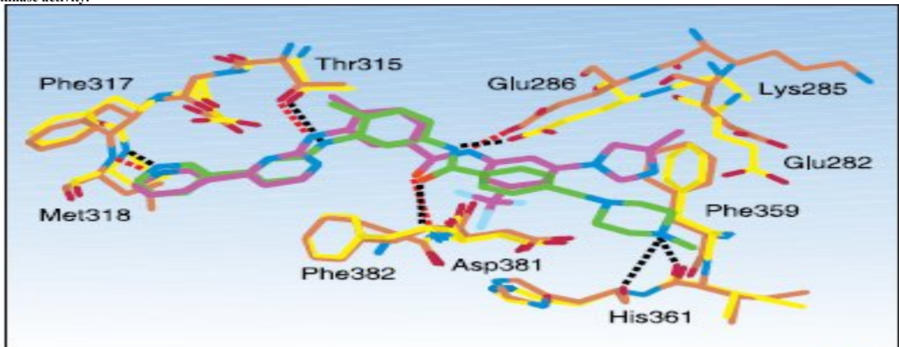
Fig. 4: Superposition of nilotinib (magenta) bound to ABLM351T (orange), and imatinib (green) bound to ABL (yellow). Hydrogen bonds within the nilotinib-ABLM351T complex are depicted as dashed red lines, whereas those in the imatinib complex are shown in black. Note that the hydrogen bonds between the piperazine ring of imatinib and Ile360 and His361 are absent from the nilotinib-ABL complex. The methyl-imidazole group of nilotinib packs in a hydrophobic pocket. (Weisberg E, Manley PW, Breitenstein W. Characterization of AMN107, a selective inhibitor of native and mutant BCR-ABL. Cancer Cell . 2005;7:129-41.)
