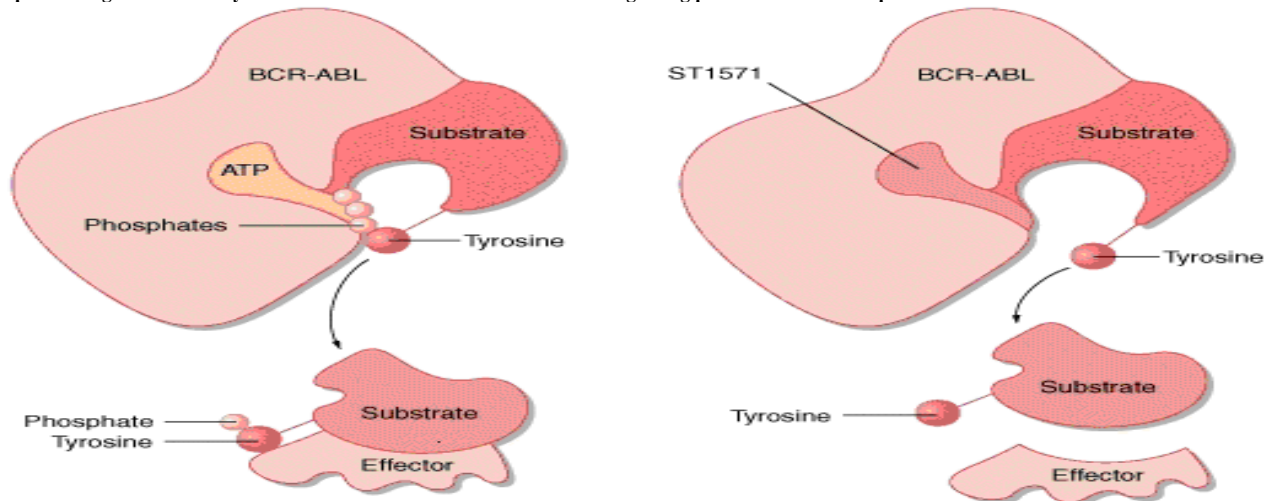
Fig. 3: Mechanism of action of imatinib. (A) The constitutively active BCR-ABL tyrosine kinase functions by transferring phosphate from ATP to tyrosine residues on various substrates to cause excess proliferation of myeloid cells characteristic of CML. (B) Imatinib blocks the binding of ATP to the BCR-ABL tyrosine kinase, thus inhibiting kinase activity.
