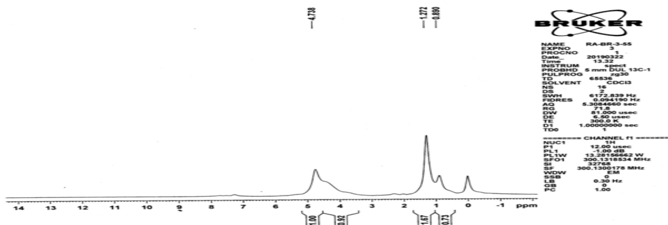
Fig. 11: ^1\text{H} NMR of isolated compound
